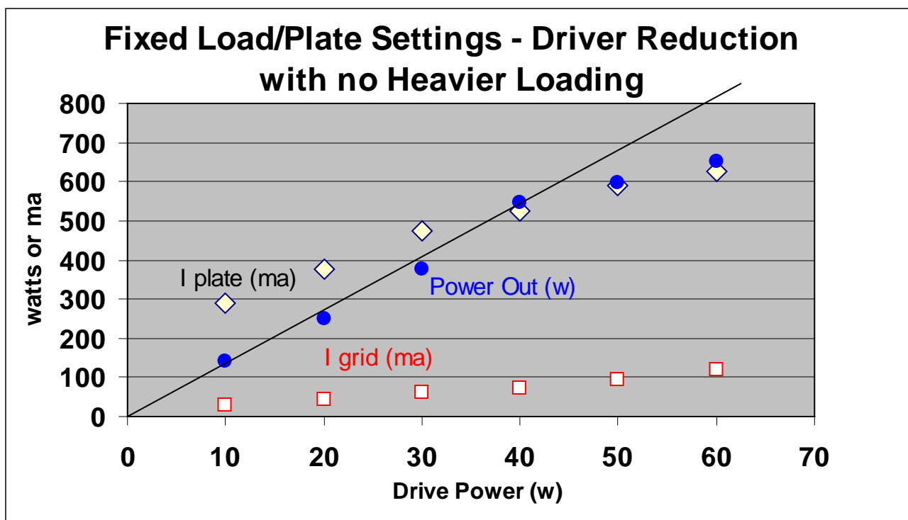
Figure 3. Effect of driver power reduction with fixed Plate/Load settings.
