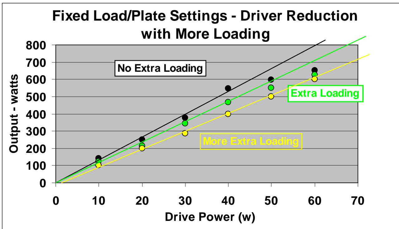
Figure 4. Effect of driver power reduction with fixed Plate/Load settings for 3 levels of loading.
