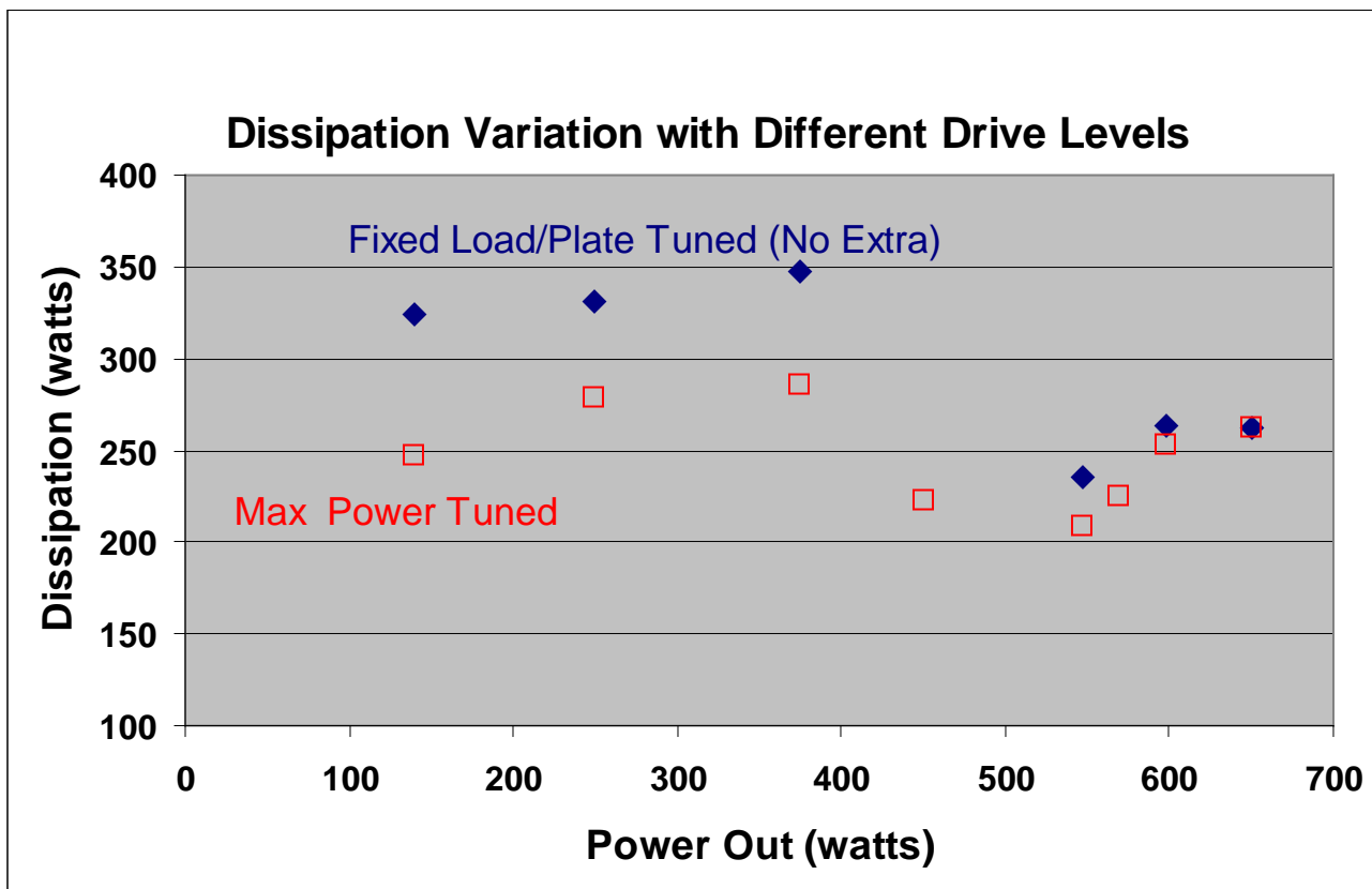
Figure 5. Variation of dissipation with drive power reduction.
