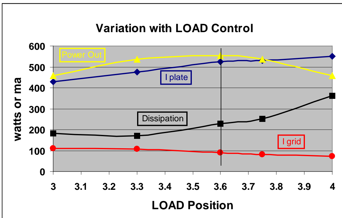
Figure 6. Effects of Load control variation (on 15 meters) about the max output with fixed 40 watts drive.
