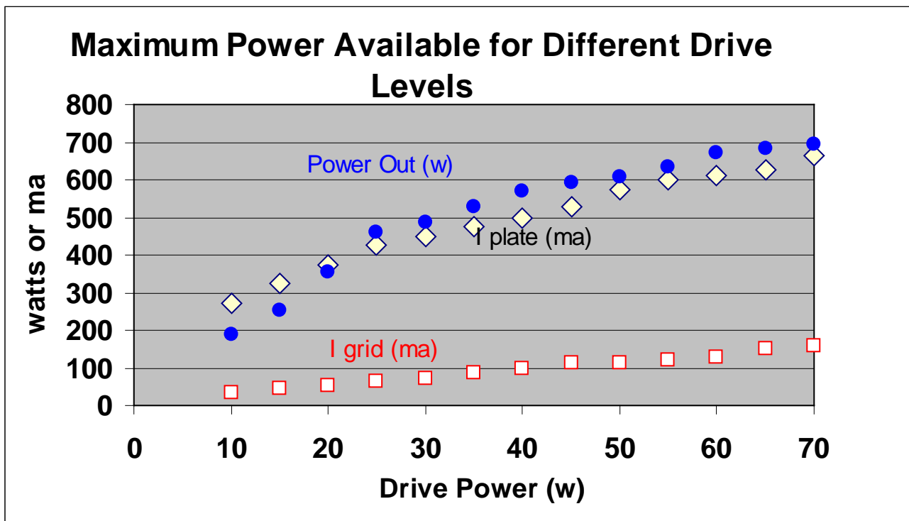
Figure 1. Maximum power out available for different drive powers (constant key down).
