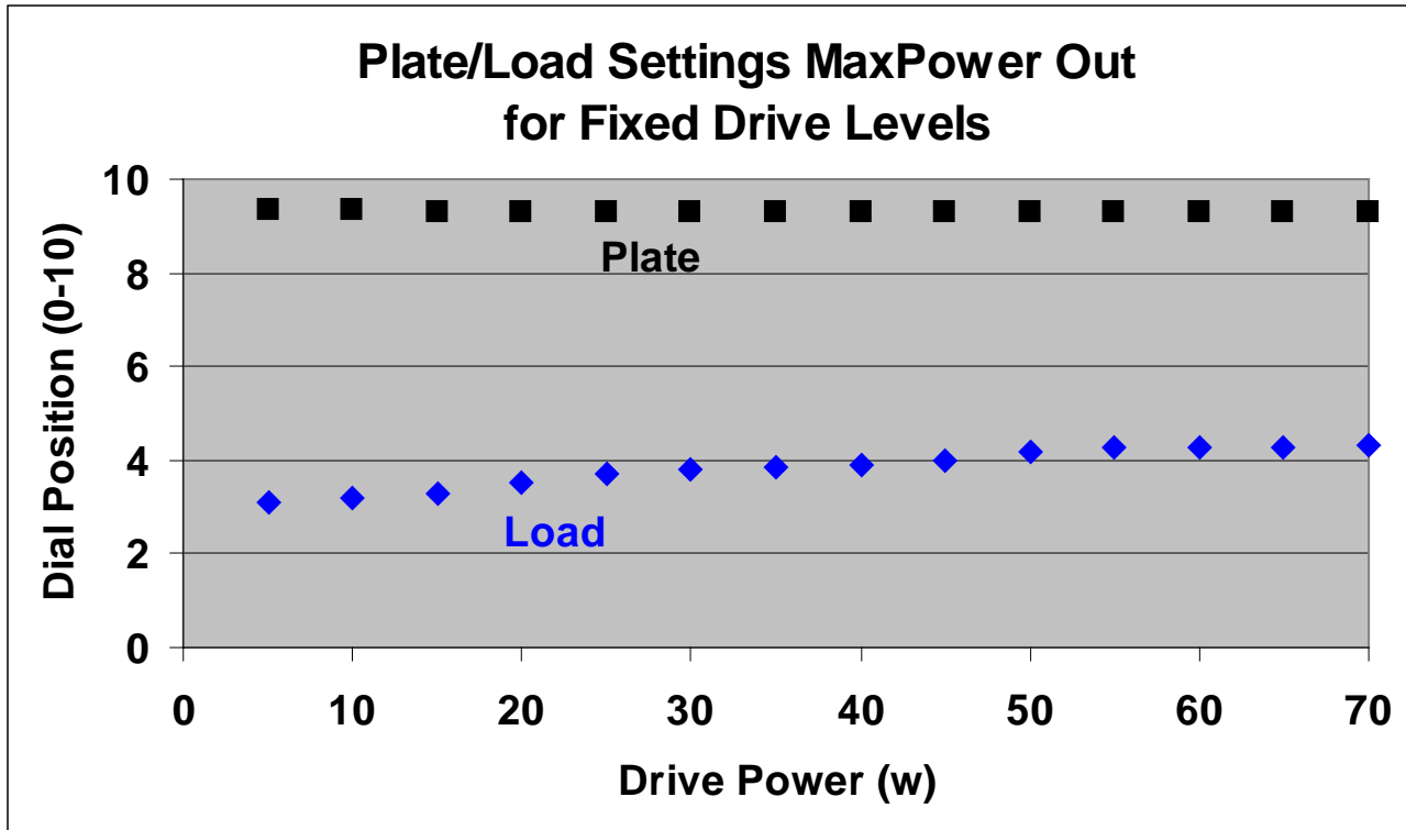
Figure 2. Plate and Load amp setting for max power out for the same conditions in the first figure.
